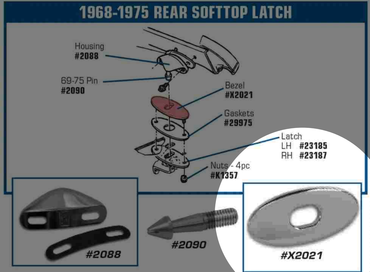
Die Casting Rear Latch Deckled Bezel made by Weser
