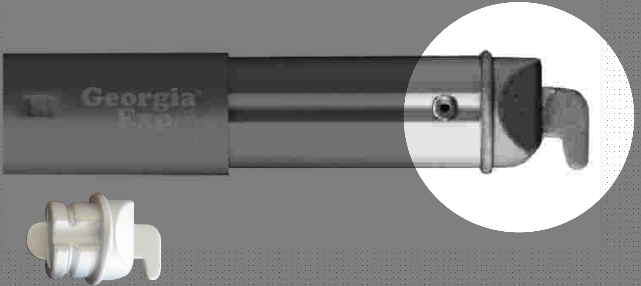
Injection Molding Nylon Hook End for Premier Drape Support made by Weser
