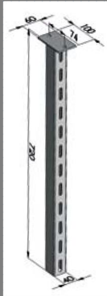
Stamped Fixed Post for Truck made by Weser
