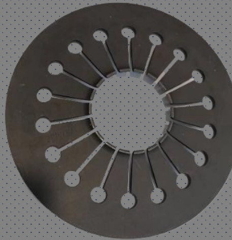
Stamping Spring Disc for BMW motor made by Weser
