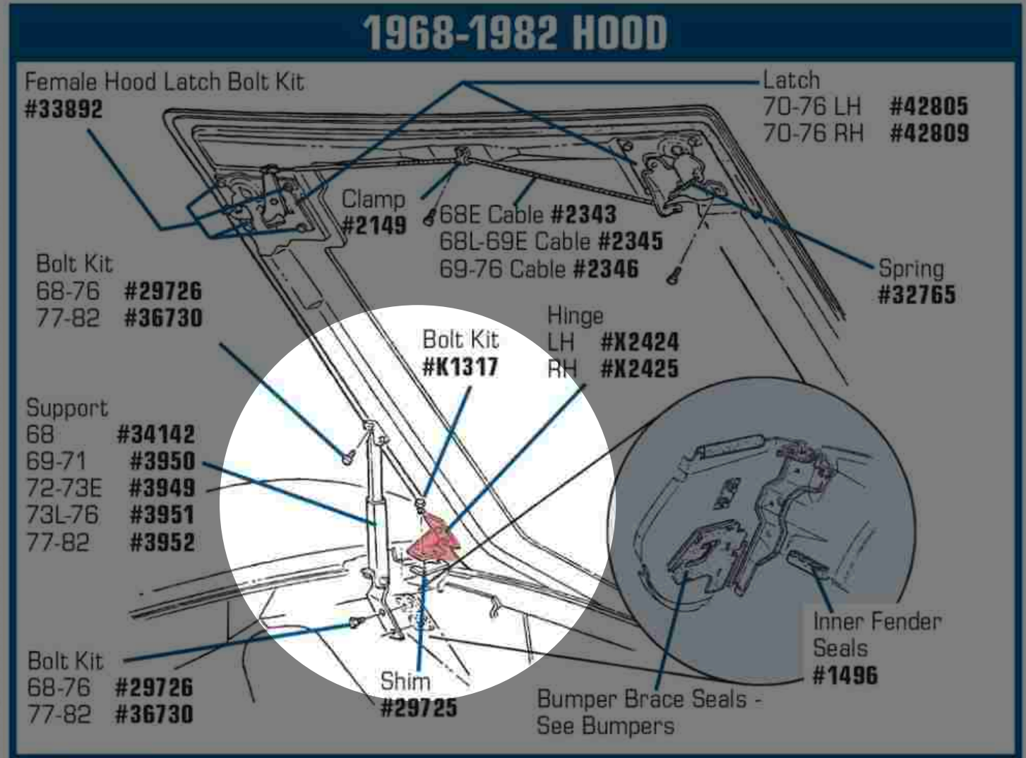
Stamp Hood Hinge made by Weser
