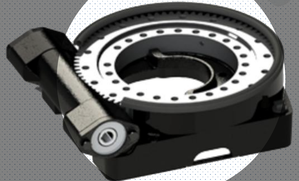
Sand Casting Square Base Mounting for Swing Drive made by Weser
